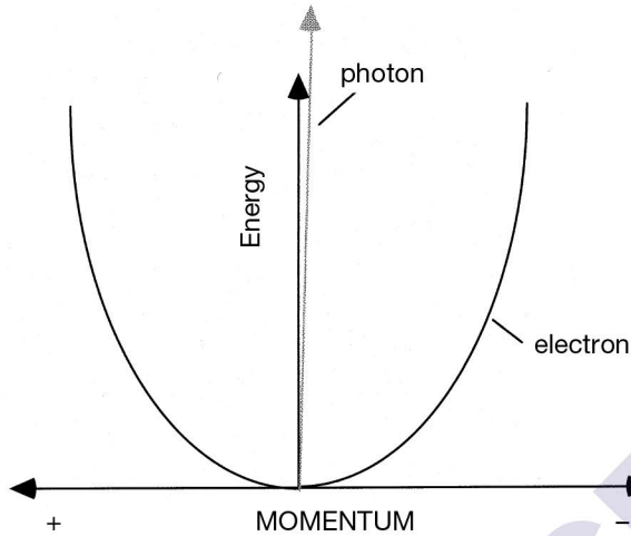
Figure 2.4. The energy of a photon is linearly proportional to its momentum. When plotted on the same graph as that for an electron, the energy–momentum relationship for a photon looks like a vertical line.
